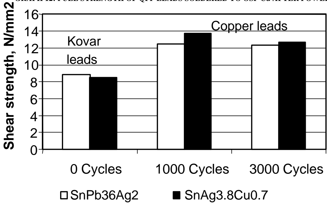
GRAPH 12: PULL STRENGTH OF QFP LEADS SOLDERED TO OSP Cu AFTER POWER CYCLING
