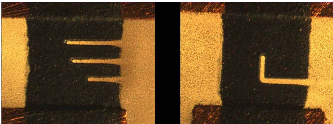
Figure 4 Laser Trim
