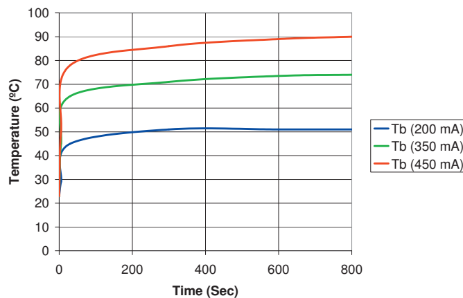
Figure 5: MCPCB Temperature
