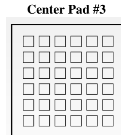
Figure 27c 1.35x1.35mm squares (10) @ 1.5mm pitch – 81% coverage
