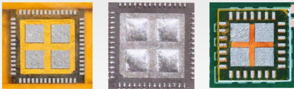
Figure 25a QFN with Stencil (8) And Solder Paste
