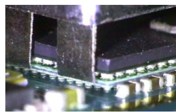
Figure 13. Tweezer Nozzle (Finetech) (Removes both Packages together)
