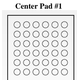
Figure 27a 1.00mm diameter (10) circles @ 1.2mm pitch – 50% coverage
