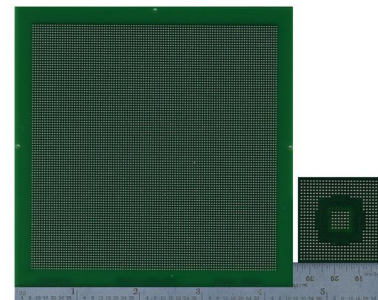
Figure 2. 114mm BGA (10,000 I/O) with 35mm BGA shown for scale
