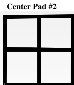
Figure 27b 3.10mm squares (10) @ 3.95mm pitch – 60% coverage
