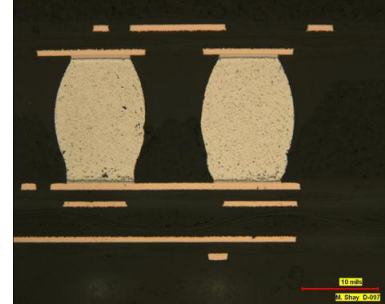
Figure 22. Cross Section showing good results (flux brushed on)
