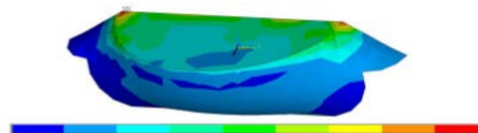
Creep strain contour in the BOL solder joint
