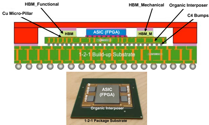
Figure 9 – SiP with organic interposer
