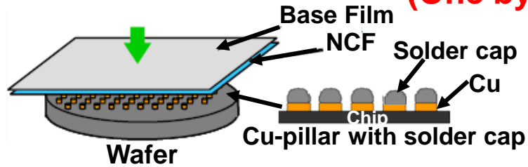
NCF Lamination for wafer
