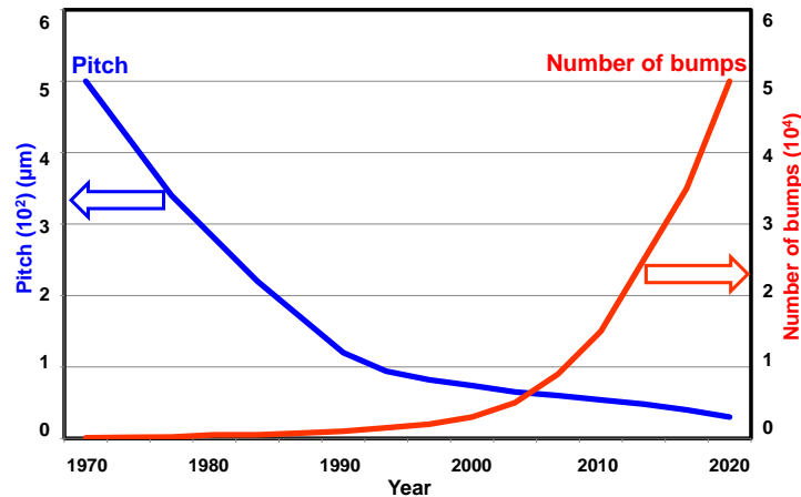
Figure 20 - Trend in flip chip bump and pitch
