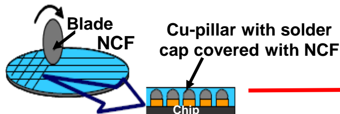
Removing based film and dicing the bumped wafer with NCF
