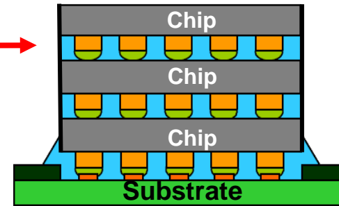
TCB with NCF
