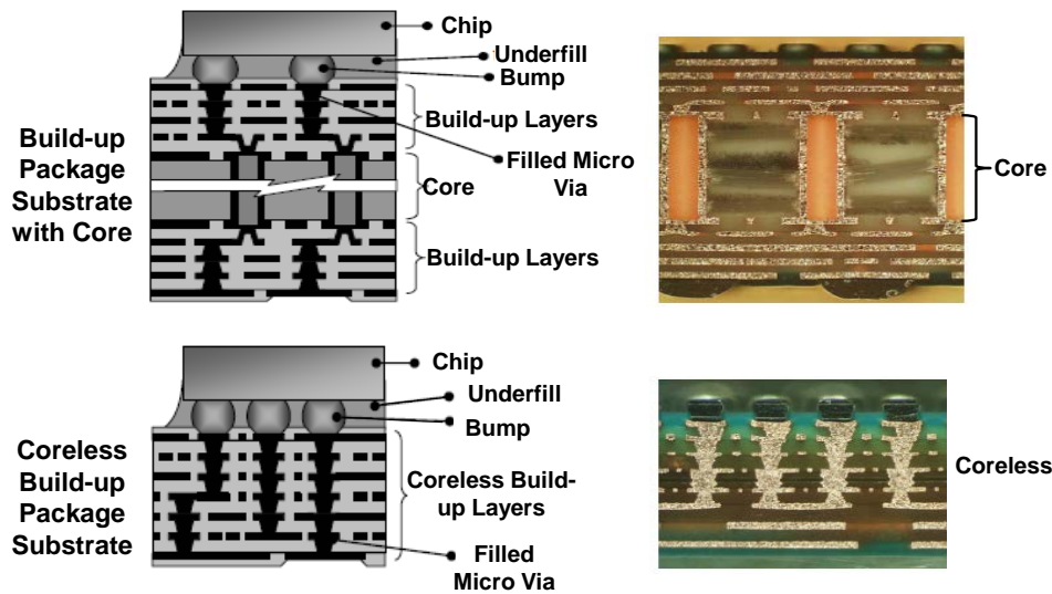
Figure 10 - (Top) flip chip on conventional build-up package substrate. (Bottom) flip chip on coreless substrate
