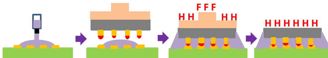
(c) TCB with High-Force of C2 Bumps (NCP)
