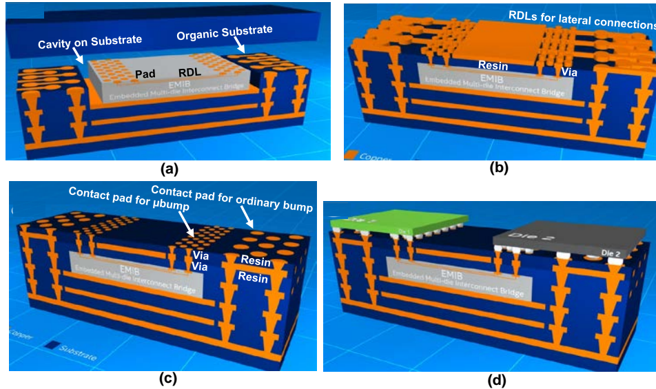
Figure 8 - Simple process flow of the EMIB technology
