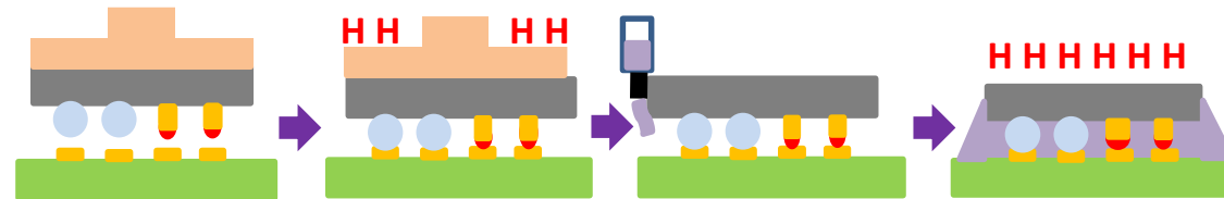
(a) Mass Reflow of C4 or C2 Bumps (CUF)
