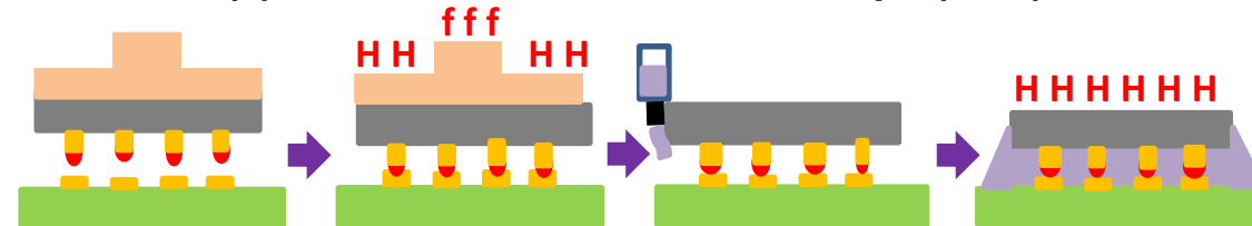
(b) TCB with Low-Force of C2 Bumps (CUF)
