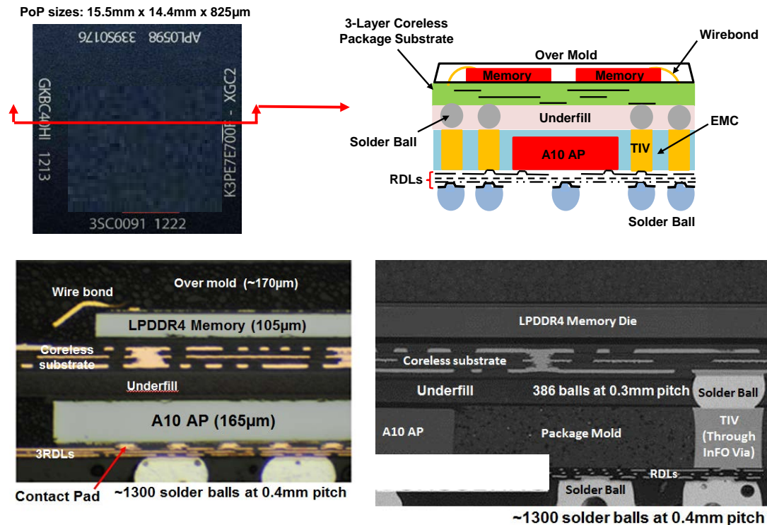
Figure 21 - PoP in production smartphone. In the bottom package, the AP is embedded in the EMC and its circuitry is fanned out through the RDLs to the PCB [63]
