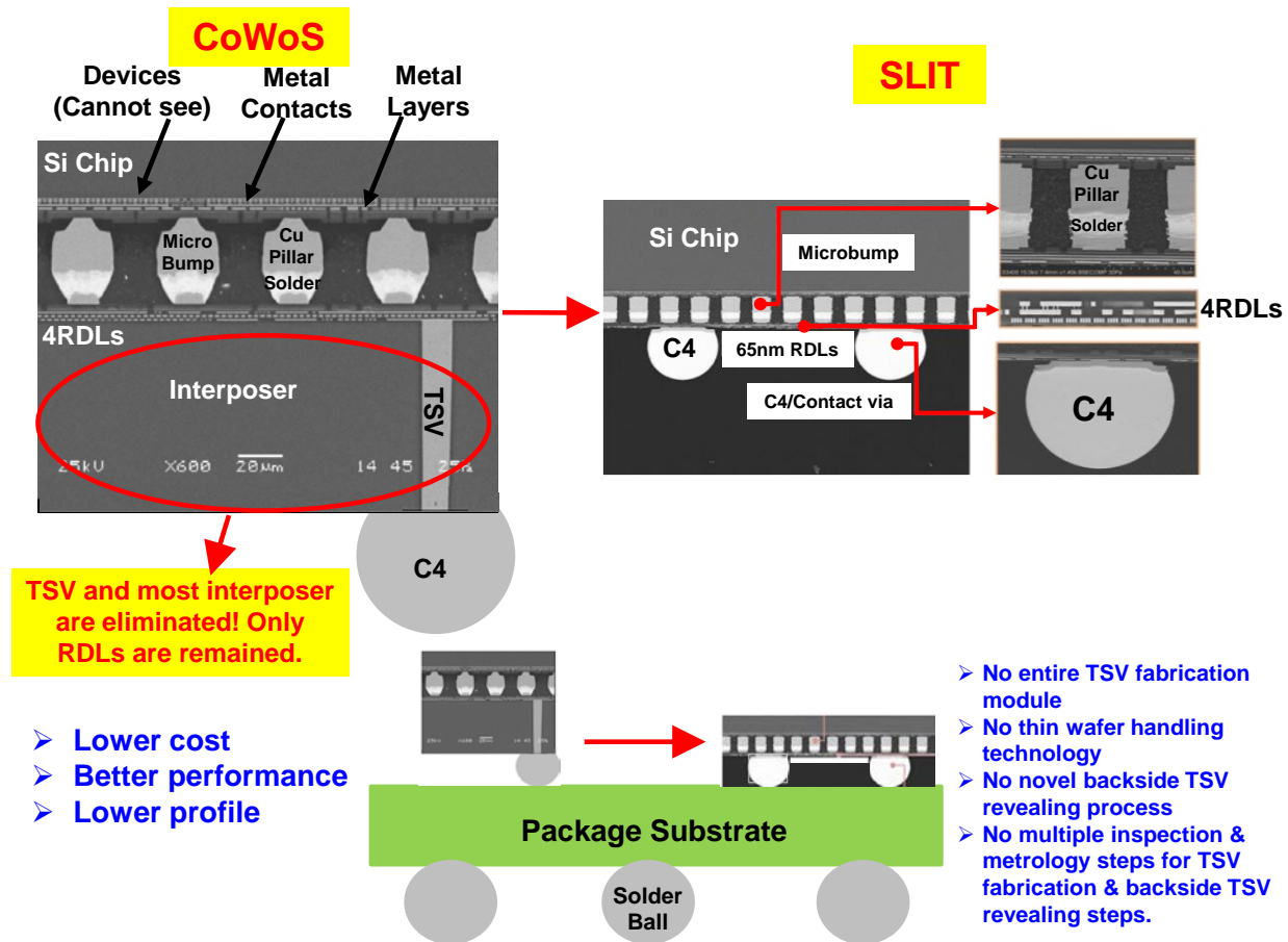
Figure 5 – CoWoS (left) and SLIT (right)
