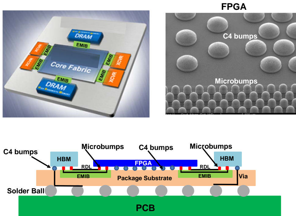
Figure 7 - High bandwidth communications between the FPBA and HBMs by EMIB
