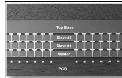
Samsung's 3D IC integration by TCB with NCF
