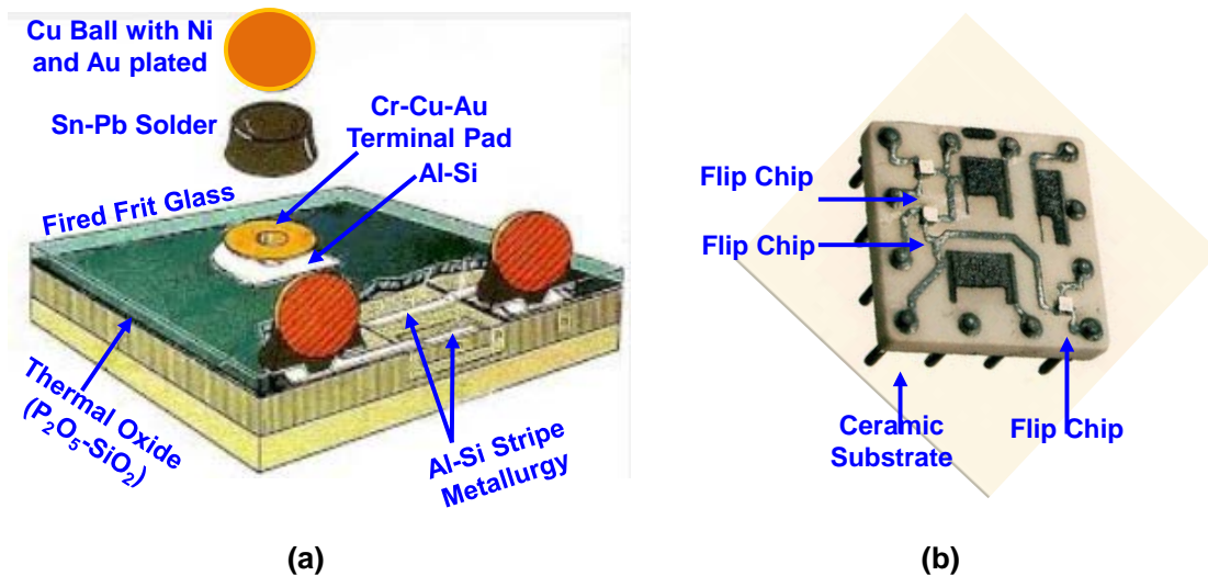
Figure 1 - (a) First flip chip component with 3 terminal transistors. (b) First flip chip assembly (3 chips) on a ceramic substrate
