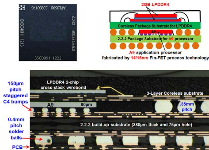
Figure - 15 PoP in a production smartphone. In the bottom package, the C4 solder bumped (AP) flip chip is mass reflowed on a 2-2-2 package substrate with an underfill, and then BGA to the PCB
