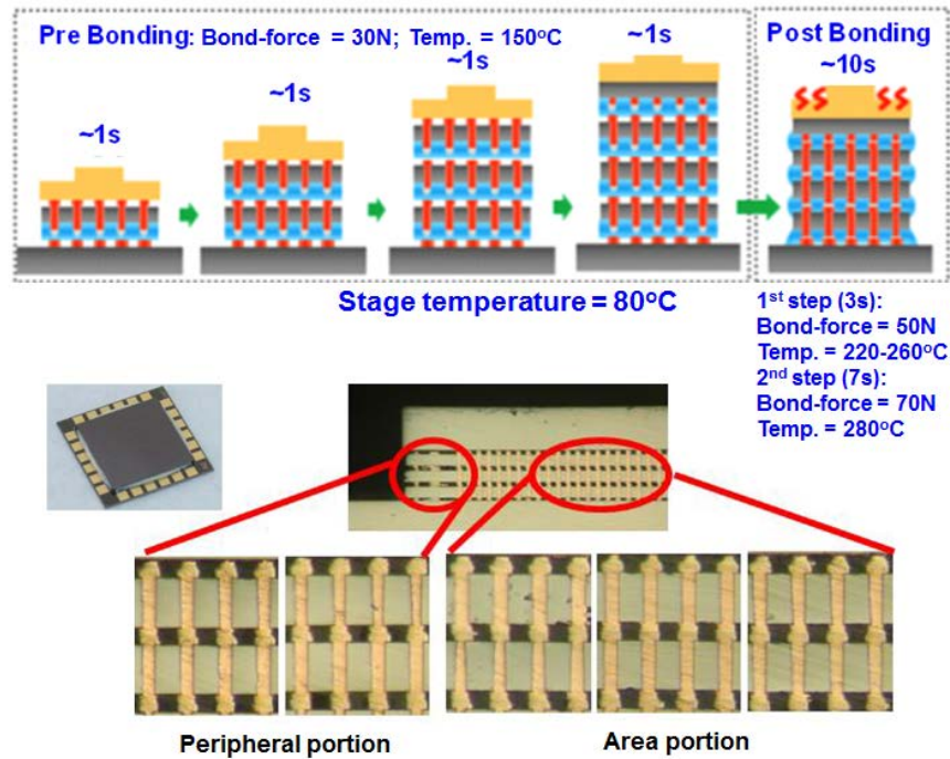
Figure 19 - Collective TCB with high-force with NCF flip chips
