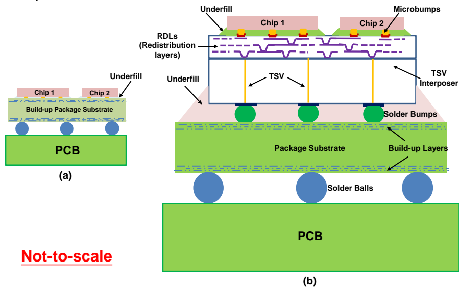
Figure 4 - (a) Build-up package substrate for flip chips. (b) Build-up substrate with TSV-interposer for flip chips Surface Laminar Circuit (SLC) Technology.
