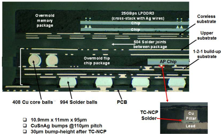
Figure 17 - PoP in a production smartphone. The C2 flip chip is TCB with high-force on a package substrate (TC-NCP)
