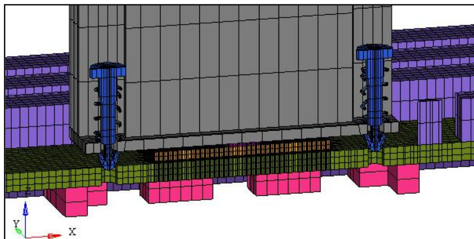
Figure 3. FEA model
