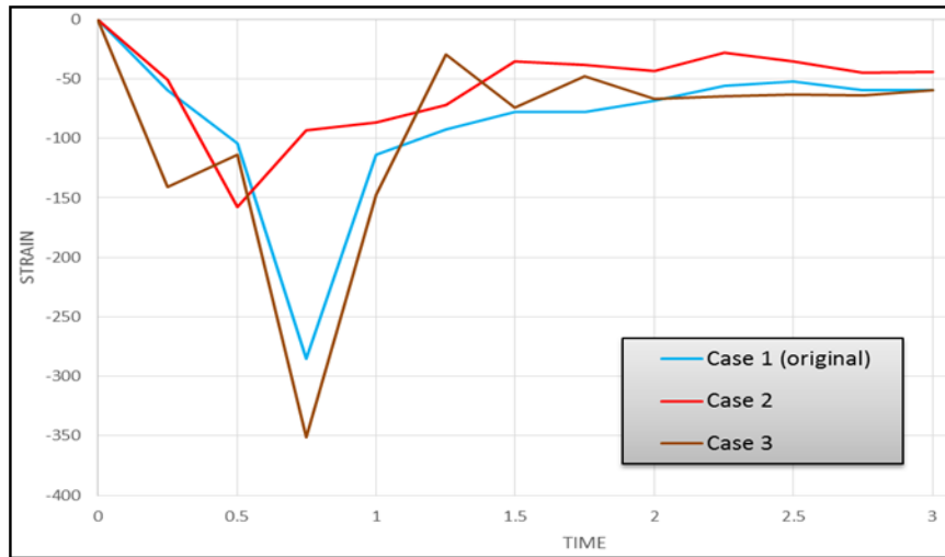
Figure 11. Max. Strain Graph (BGA location change)
