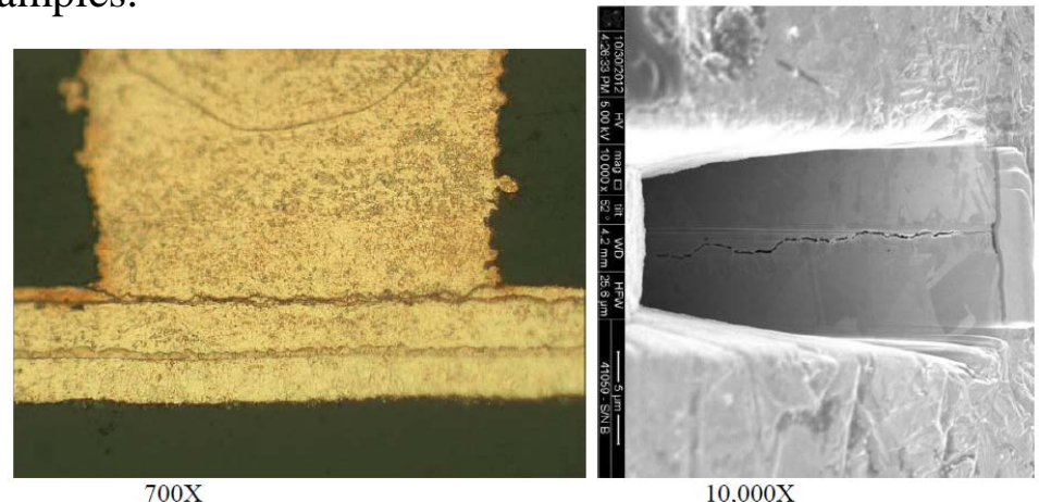
Cross-section and SEM Images of Failed Micro Voids [ref: IPC APEX Conference, 2014 ]
