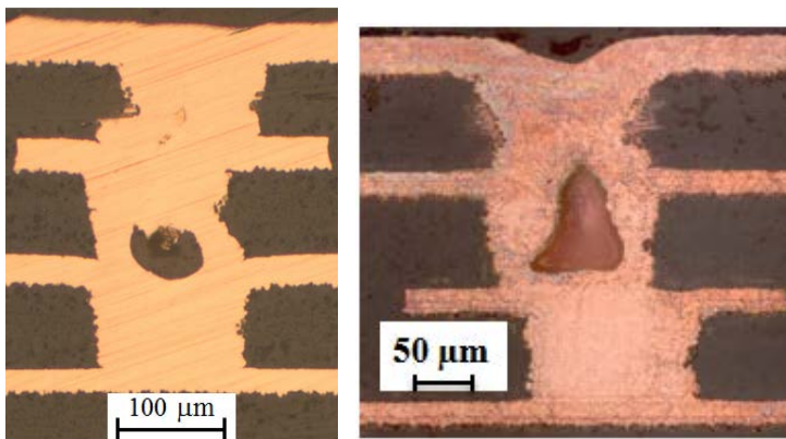
Examples of Microvias with Voids
